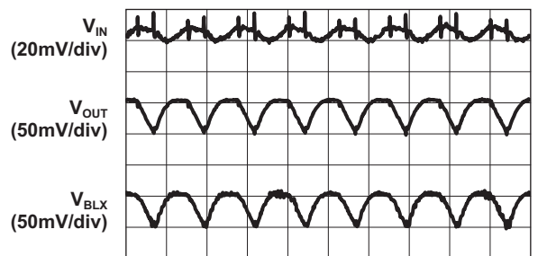
Time (1µs/div)
