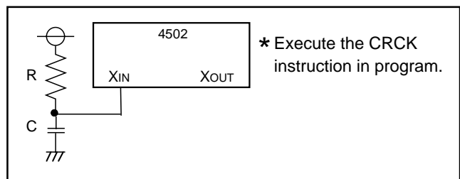
Fig. 46 External RC oscillation circuit
