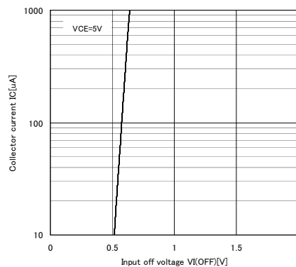
Collector current-Input off voltage
