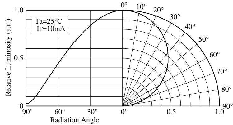
■ Directivity (NECW425B)
