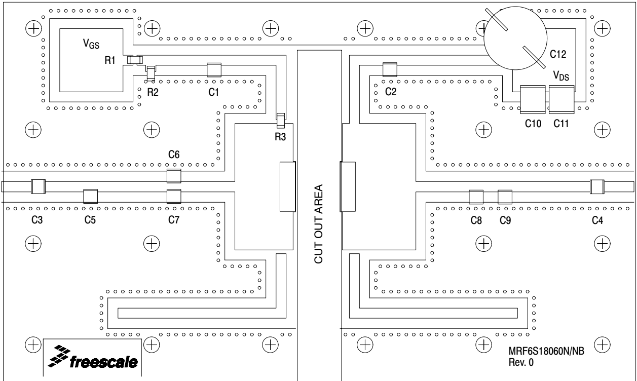
Figure 17. MRF6S18060NR1(NBR1) Test Circuit Component Layout — 180 MHz
