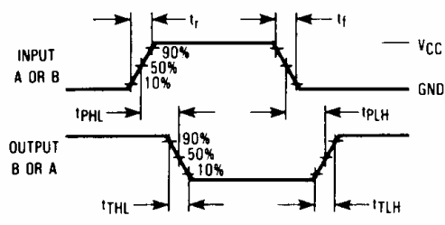
Figure 1. Switching Waveforms
