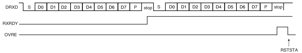
Figure 20-7. Receiver Overrun
