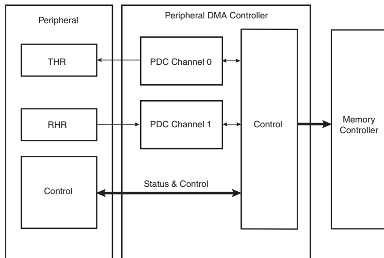
Figure 15-1. Block Diagram
