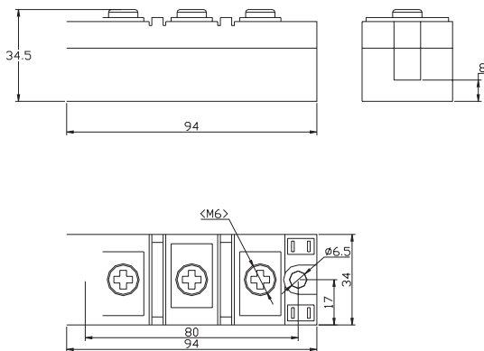
Fig. 8 - Outline Characteristics
