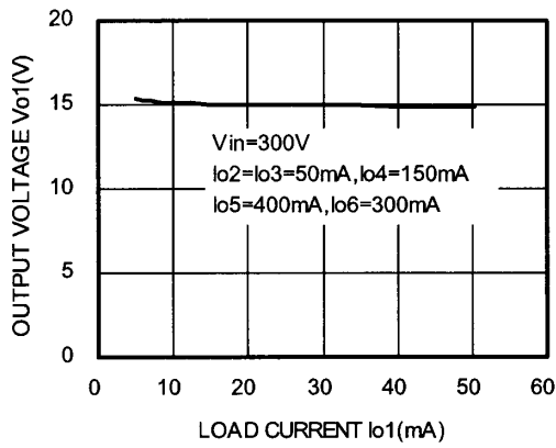
Vo1 OUTPUT VOLTAGE VS. LOAD CURRENT CHARACTERISTICS
