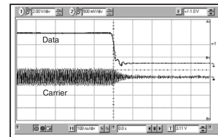
Figure 6: Typical Oscillator Turn-Off Time
