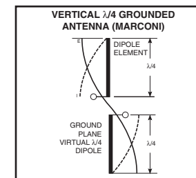
Figure 21: Dipole Antenna
