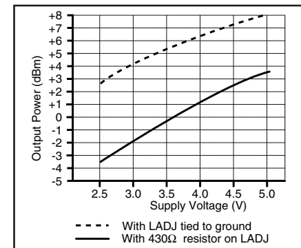
Figure 4: Output Power vs. Supply Voltage
