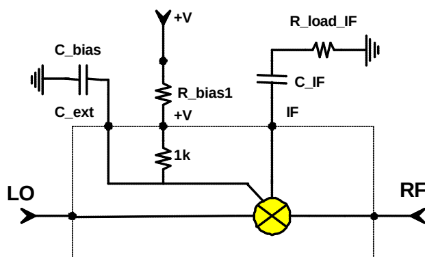
Recommended external bias and IF configuration
