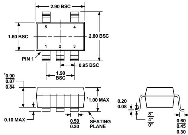
*COMPLIANT TO JEDEC STANDARDS MO-193-AB WITH THE EXCEPTION OF PACKAGE HEIGHT AND THICKNESS. Figure 50. 5-Lead Thin Small Outline Transistor Package [TSOT] (UJ-5) Dimensions shown in millimeters
