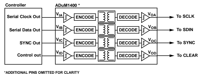
Figure 16. Isolated Interface
