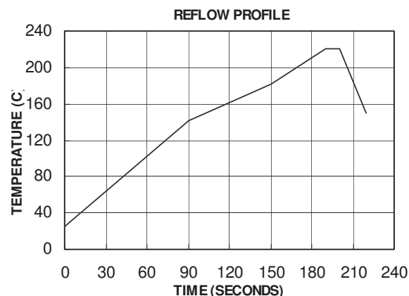
Figure 14 VPOL5A-12-SMT Reflow Profile
