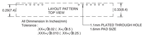
Figure 8. Recommended VPOL20A-12W-SIP Footprint
