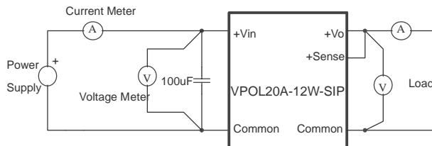
Figure 13. VPOL20A-12W-SIP Series Test Setup
