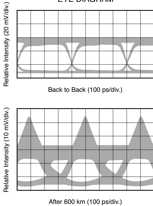
EYE DIAGRAM
