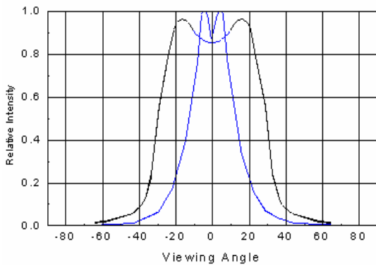
Relative Intensity vs. Angle Displacement
