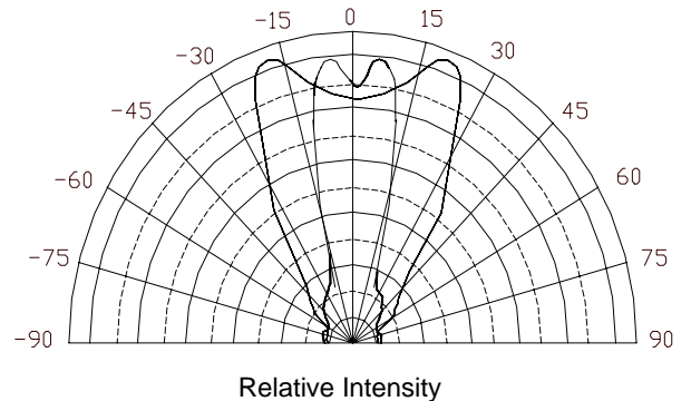
Relative Intensity vs. Off Axis Angle
