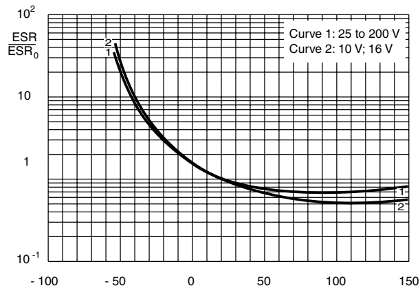
Case \varnothing D x L = 6.5 x 18 to 15 x 30 mm ESR 0 = typical at 20 °C, 100 Hz
