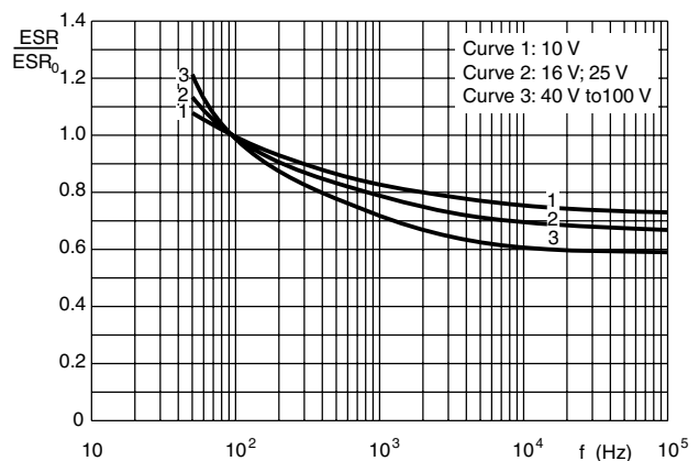
Case \varnothing D x L = 10 x 30 to 21 x 38 mm ESR 0 = typical at 20 °C, 100 Hz
