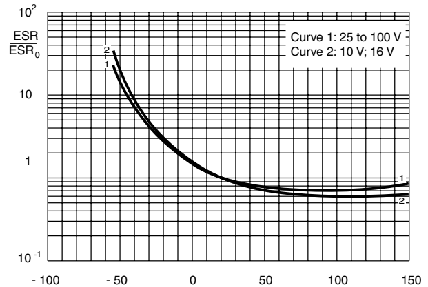
Case \varnothing D x L = 18 x 30 to 21 x 38 mm ESR 0 = typical at 20 °C, 100 Hz
