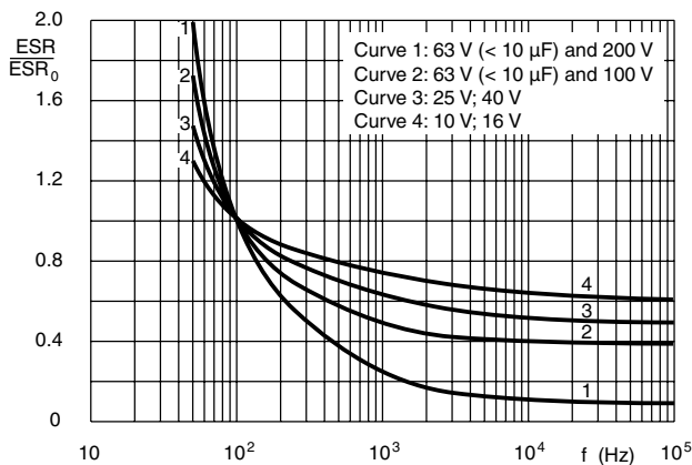
Case \varnothing D x L = 6.5 x 18 to 10 x 25 mm ESR 0 = typical at 20 °C, 100 Hz
