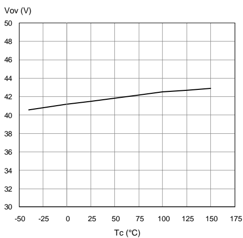
Figure 17. Overvoltage Shutdown
