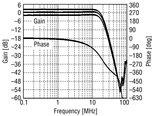
Figure 12. Gain and Phase characteristics (half fc mode, FCDDATA = 227)
