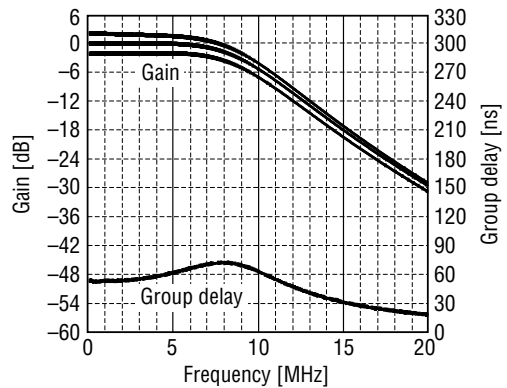
Figure 15. Gain and Group delay characteristics (CH = Y/C)
