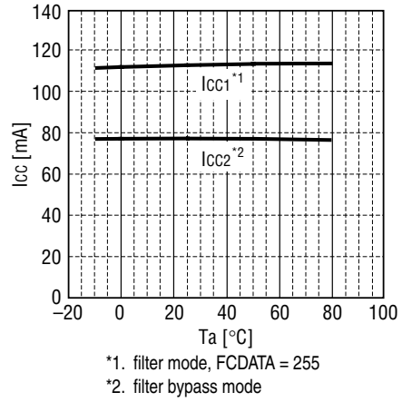
Figure 17. I_{CC1,2} vs. T_a
