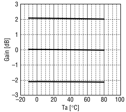
Figure 21. Gain vs. T_a
