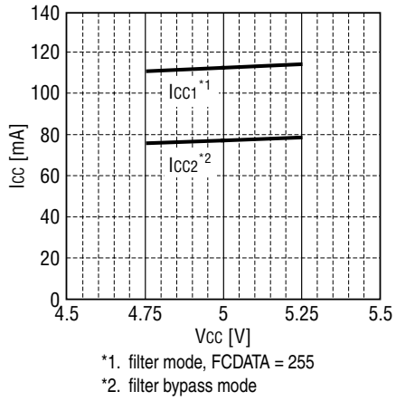
Figure 16. I_{CC1,2} vs. V_{CC}
