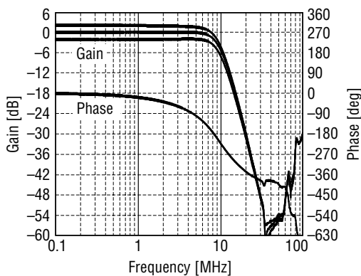
Figure 14. Gain and Phase characteristics (CH = Y/C)
