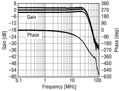
Figure 10. Gain and Phase characteristics (standard fc mode, FCDDATA = 227)
