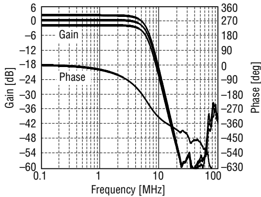
Figure 6. Gain and Phase characteristics (standard fc mode, FCDDATA = 10)
