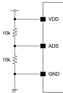
Figure 3. Slave address 4Ah setting
