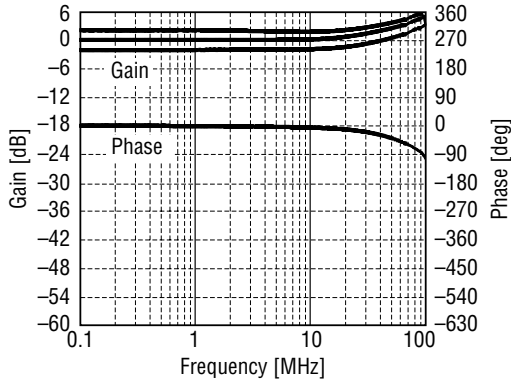
Figure 4. Gain and Phase characteristics (filter bypass mode)
