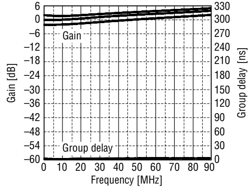
Figure 5. Gain and Group delay characteristics (filter bypass mode)
