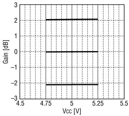
Figure 20. Gain vs. V_{CC}
