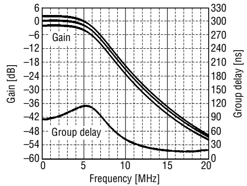
Figure 7. Gain and Group delay characteristics (standard fc mode, FCDDATA = 10)
