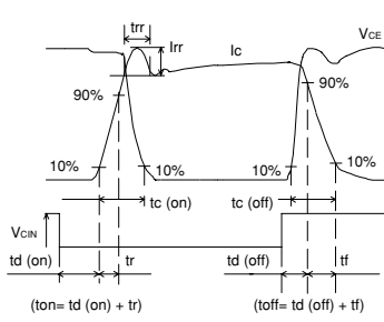
Fig. 3 Switching time Test circuit and waveform
