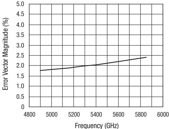
EVM vs. Frequency @ P OUT = 15 dBm
