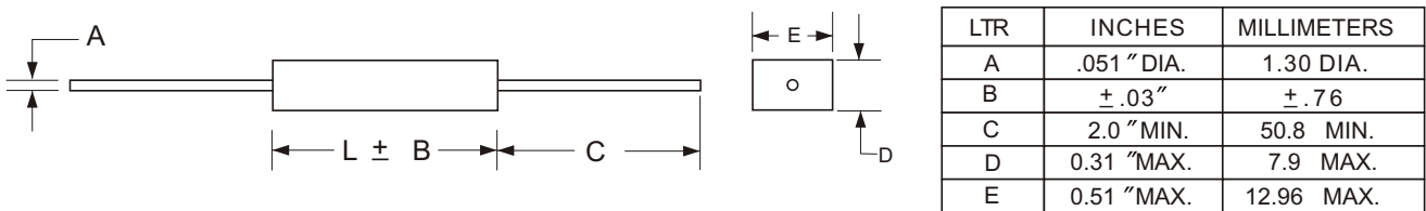
FIG.3 PACKAGE STYLE
