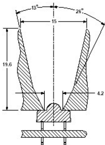
Figure 5.26 Linear profile approximation of a parabolic reflector ( f = 0.66 mm).
