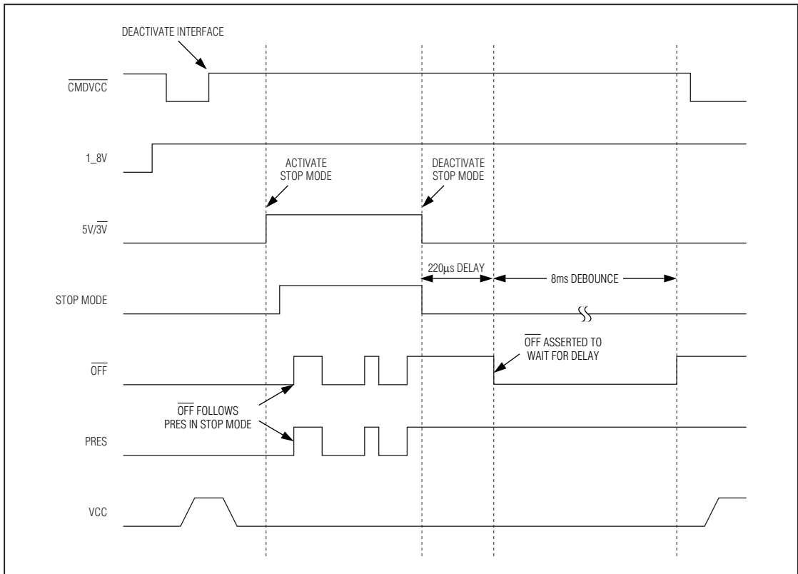
Figure 8. Stop-Mode Sequence
