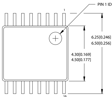
Figure 12. 16-lead TSSOP 4.40 MM Body Z16.173
