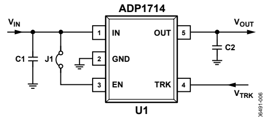
Figure 6. ADP1714 Fixed Output with Tracking
