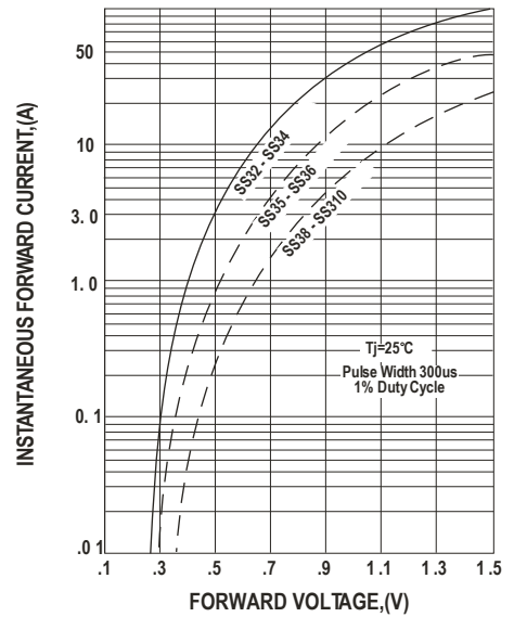
FIG.2-TYPICAL FORWARD CHARACTERISTICS
