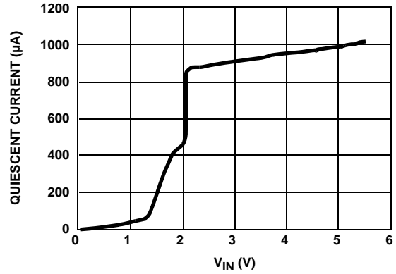
FIGURE 11. QUIESCIENT CURRENT vs V_{IN}
