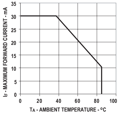
Figure 8. Forward current vs. ambient temperature.
