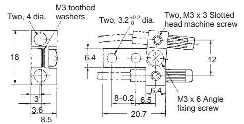
E39-F3A Reflective Lens Unit (for the E32-D32)
