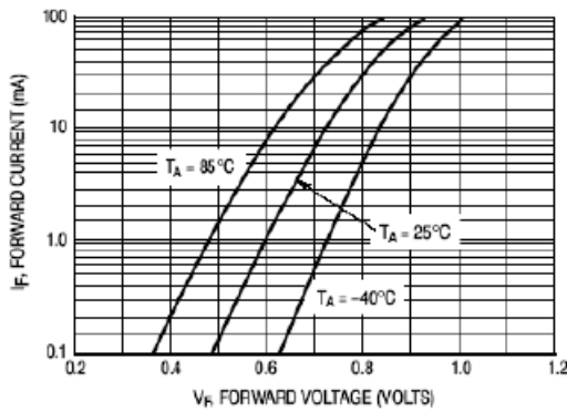
Figure 1. Forward Voltage
