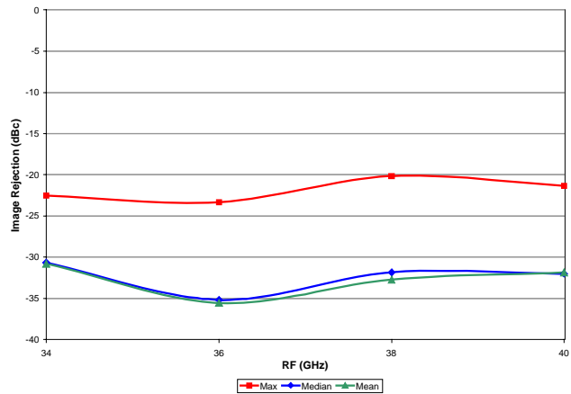
XM1002-BD, LSB Image Rejection (6566 devices)
