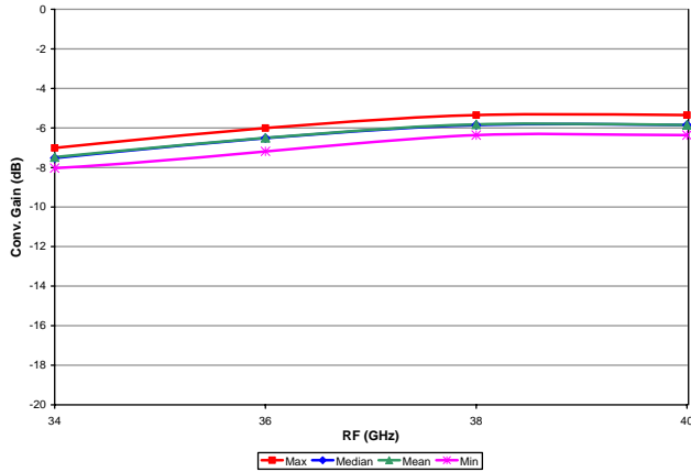
XM1002-BD, USB Conversion Gain (6566 devices)
