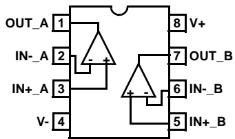
ISL28248 (8 LD SOIC) TOP VIEW
