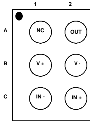
ISL28148 (6 LD WLCSP) TOP VIEW
