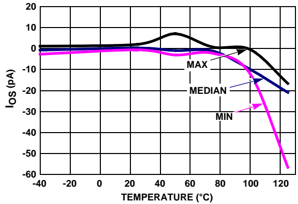
FIGURE 33. I_{OS} vs TEMPERATURE V_+ , V_- = \pm 1.2V
