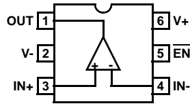
ISL28148 (6 LD SOT-23) TOP VIEW
