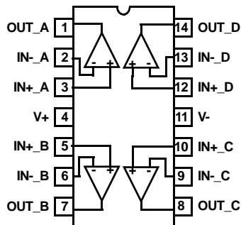
ISL28448 (14 LD TSSOP) TOP VIEW
