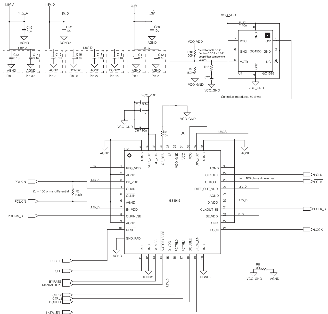
Figure 4-1: GS4915 Typical Application Circuit
