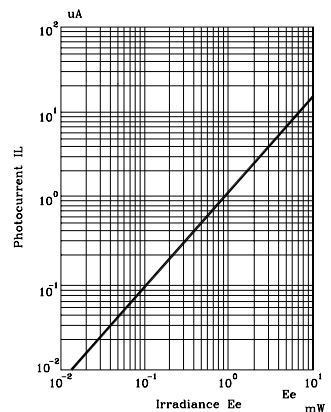
Fig.6 PHOTOCURRENT VS IRRADIANCE = 940 nm
