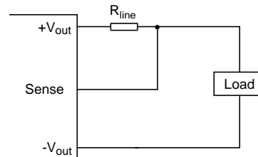
Fig.3 Sense Connection
