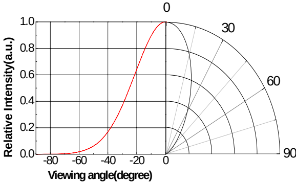
Relative Intensity vs. Displacement Angle
