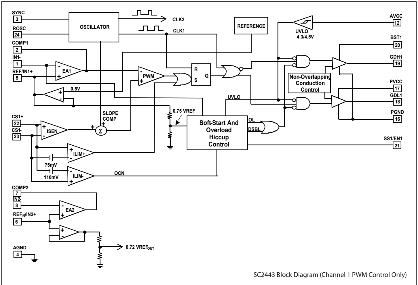
Figure 1. SC2443 Block Diagram
