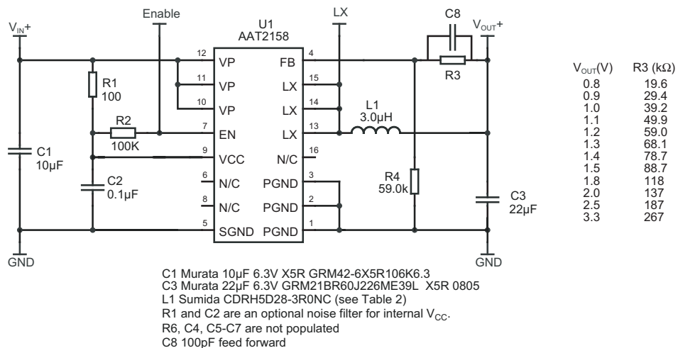
Figure 3: AAT2158 Evaluation Schematic.
