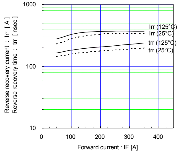
Reverse recovery characteristics (typ.) Vcc=900V, VGE=±15V, Rg=2.2Ω
