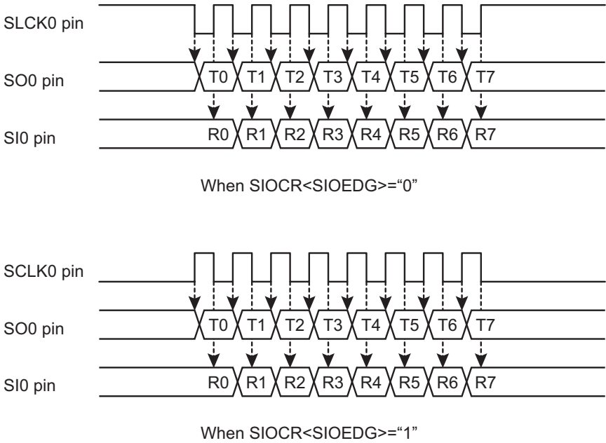
Figure 17-2 Transfer Edge
