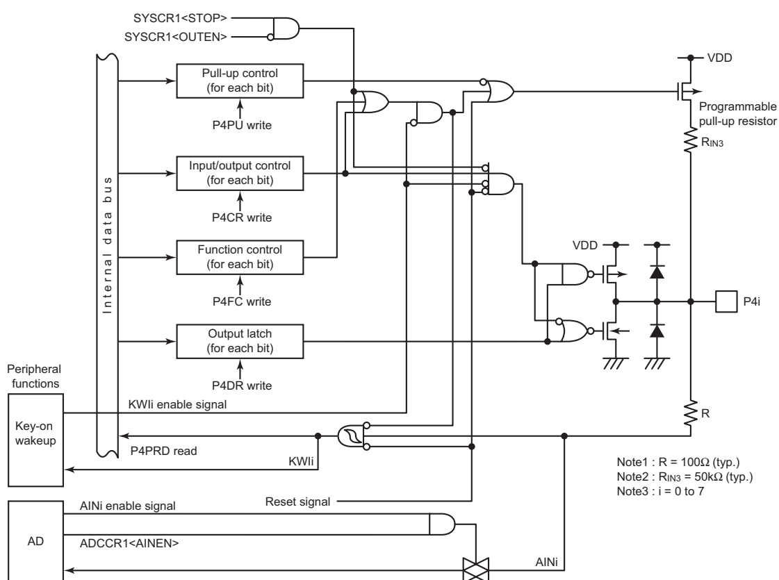
Figure 8-6 Port P4
