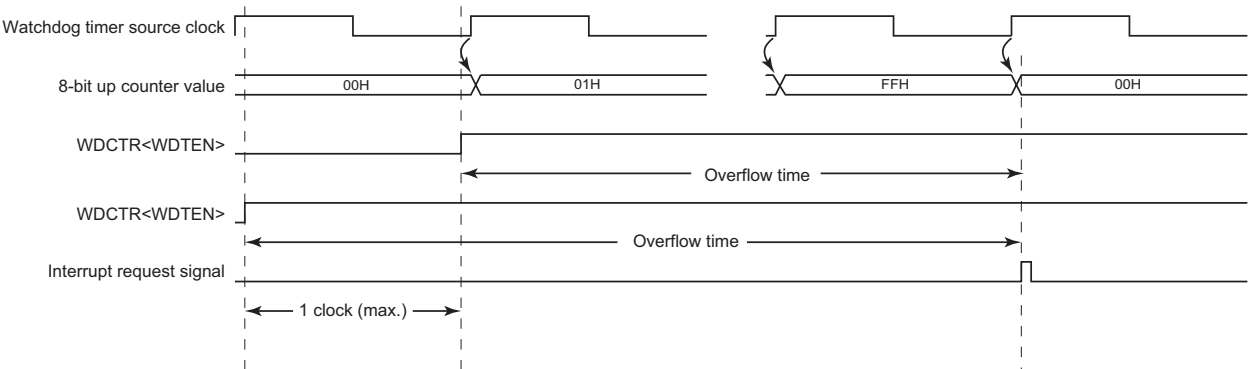
Figure 5-2 WDCTR<WDTEN> Set Timing and Overflow Time
