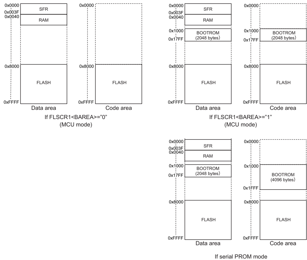
Figure 22-3 Memory Mapping
