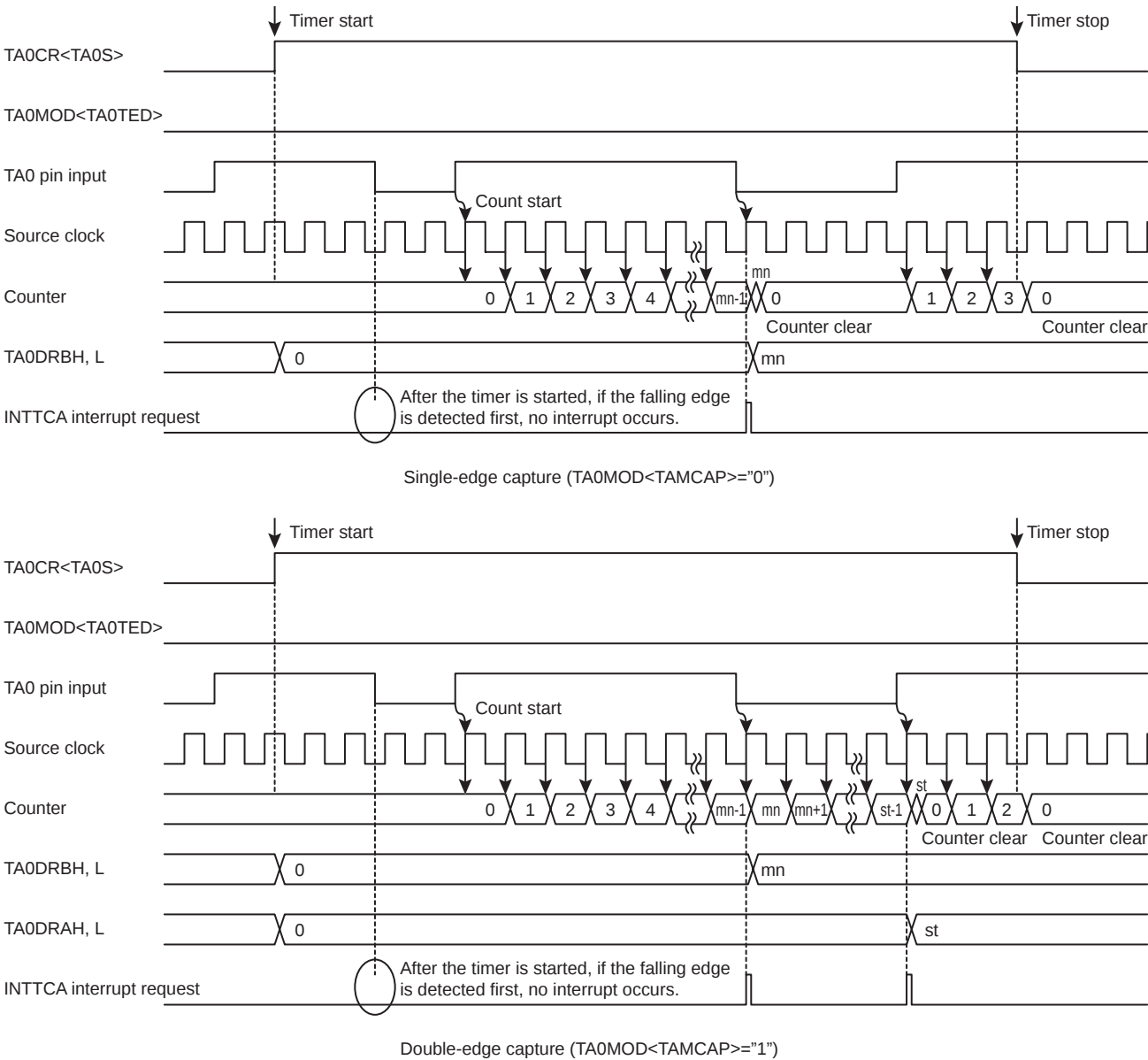
Figure 13-7 Pulse Width Measurement Mode Timing Chart
