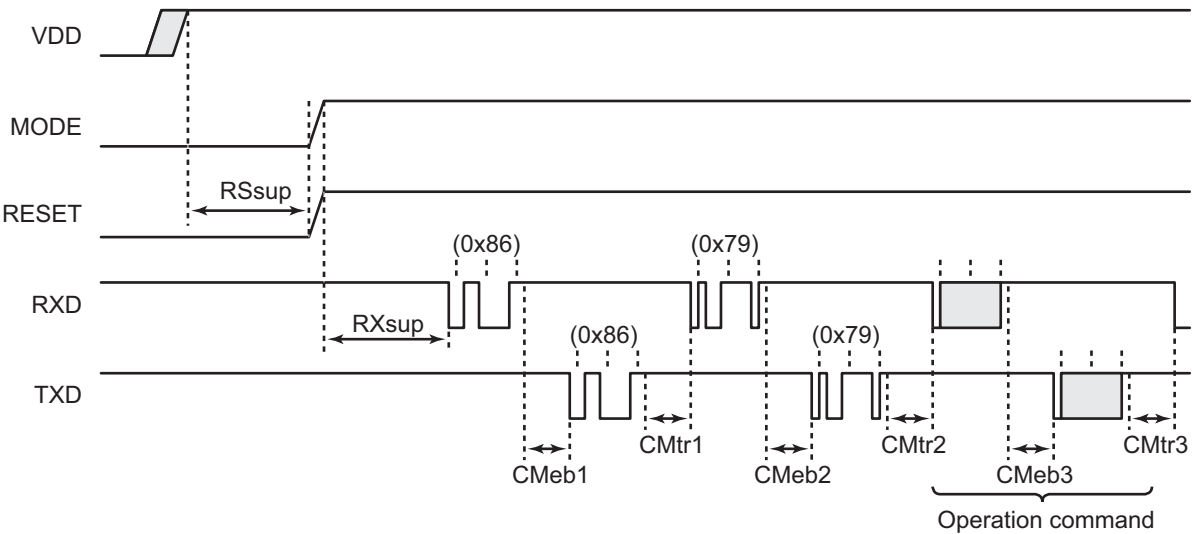
Figure 22-6 Reset Timing
