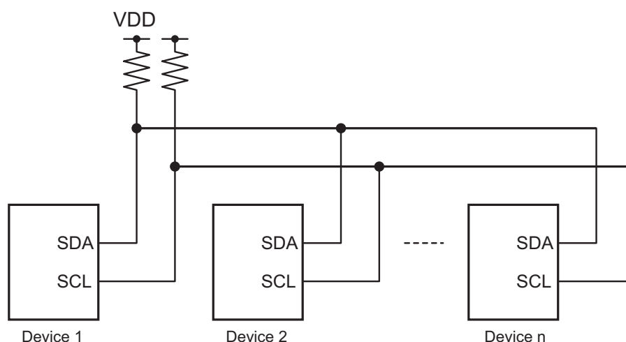
Figure 18-1 Device Connections
