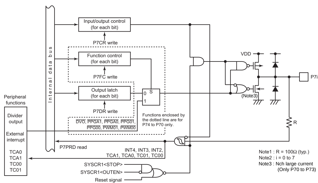
Figure 8-7 Port P7
