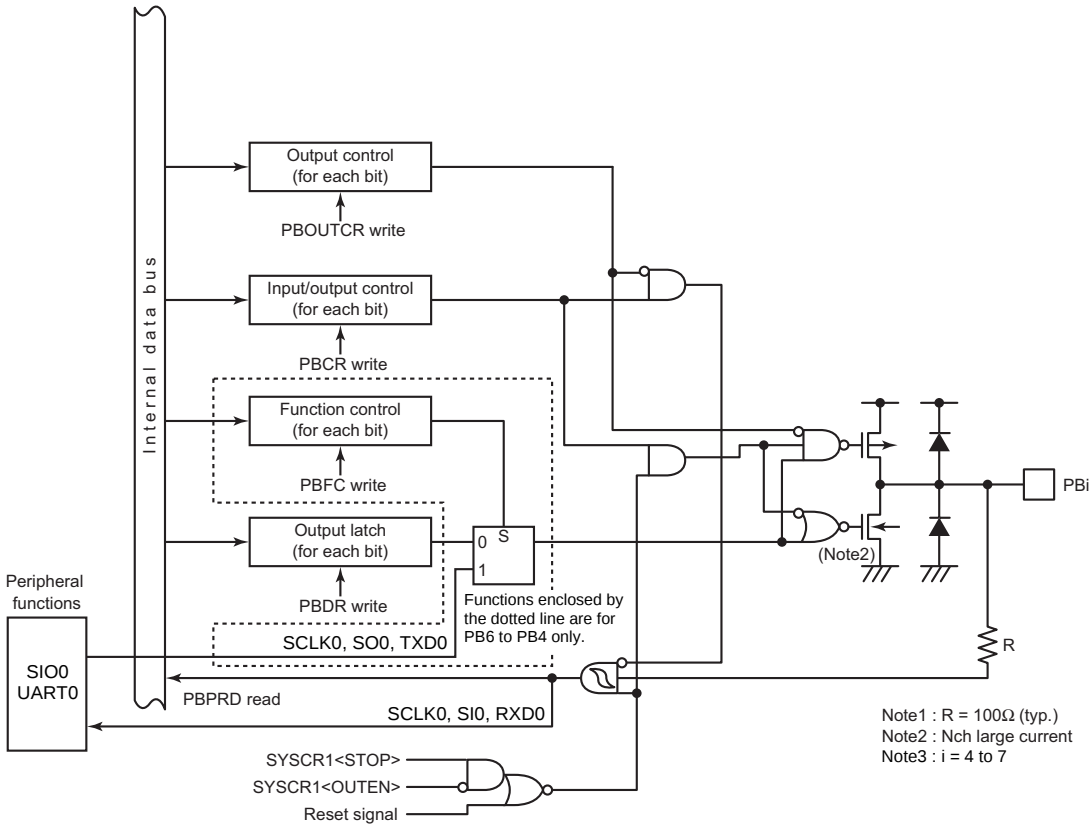
Figure 8-10 Port PB
