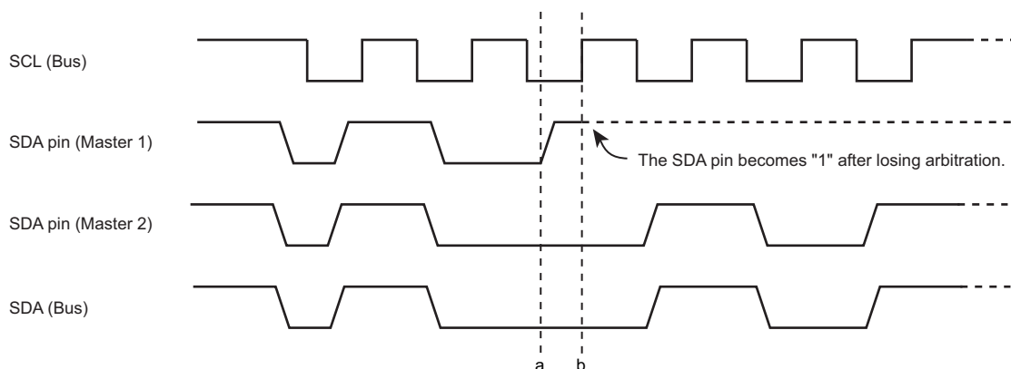
Figure 18-12 Arbitration Lost
