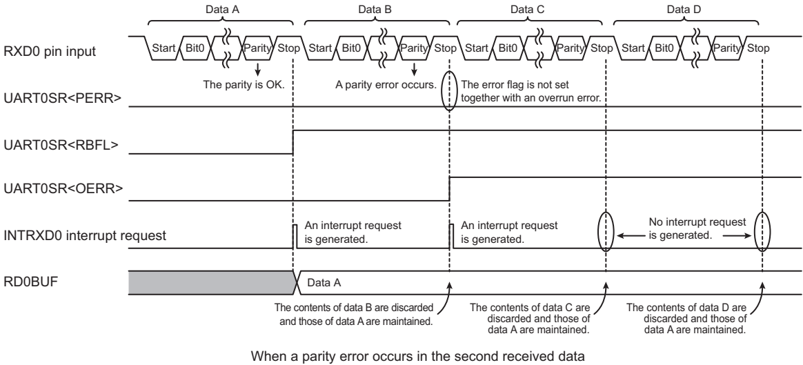
Figure 16-13 Framing/Parity Error Flags When an Overrun Error Occurs
