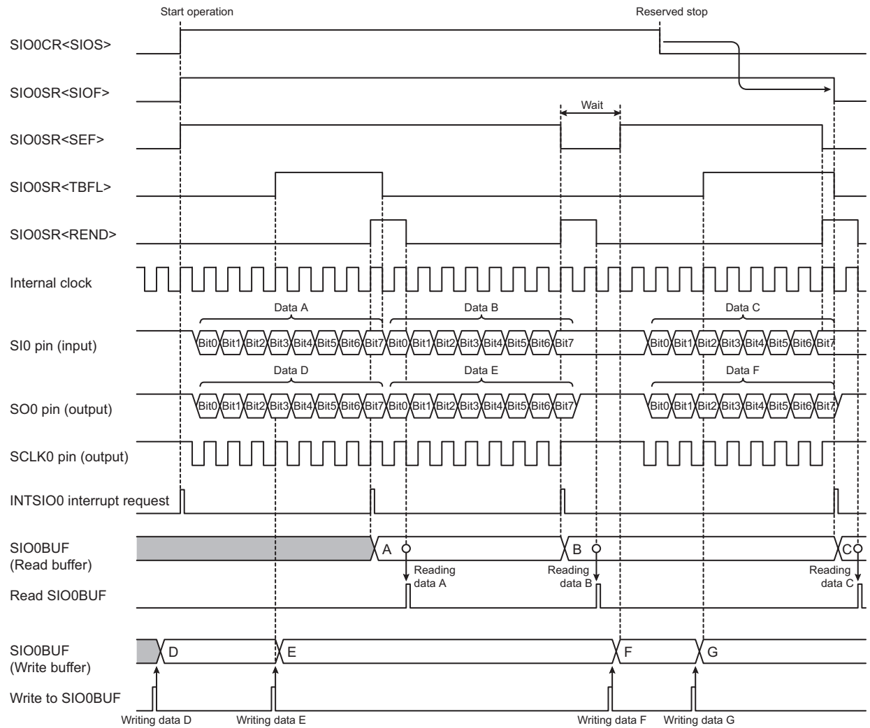
Figure 17-13 8-bit Transmit/Receive Mode (Internal Clock and Reserved Stop)
