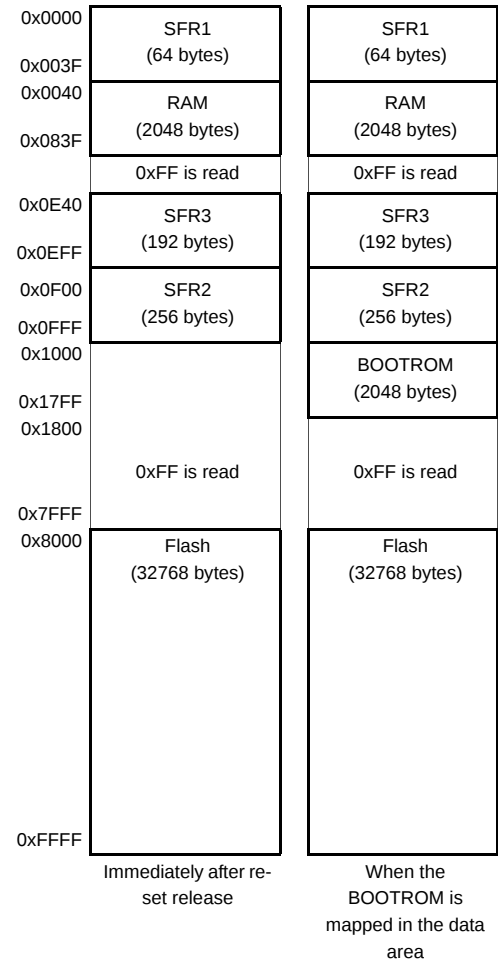
Figure 2-2 Memory Map in the Data Area
