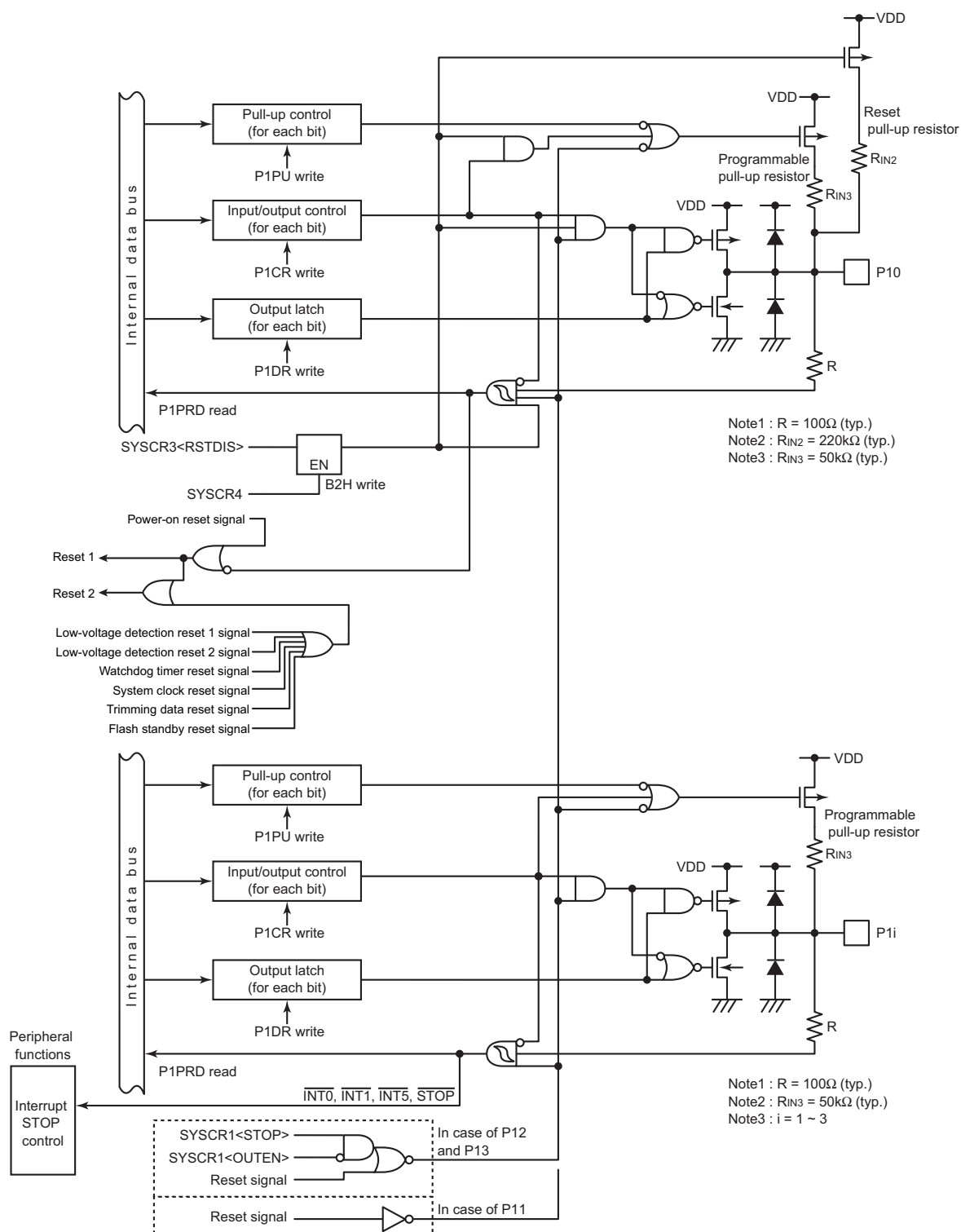
Figure 8-4 Port P1
