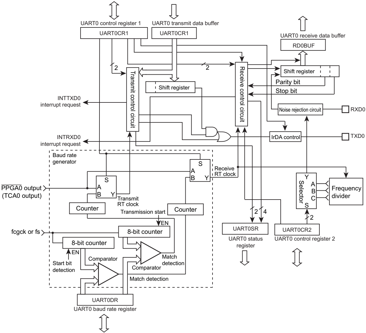
Figure 16-1 Asynchronous Serial Interface (UART)
