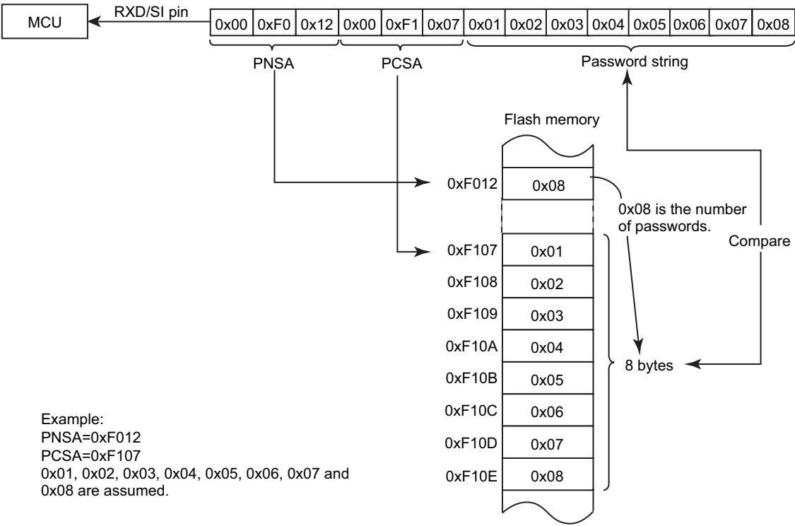
Figure 22-4 Password Structure (Example of a Password Transmitted)
