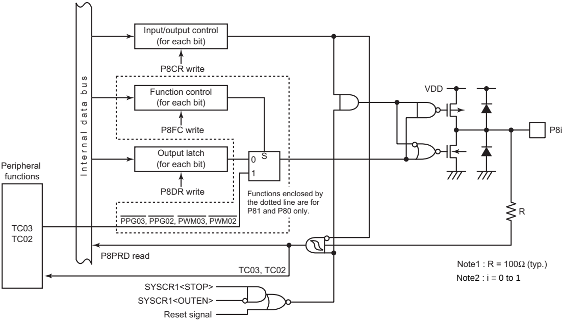
Figure 8-8 Port P8
