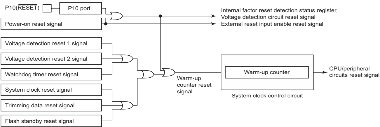
Figure 2-14 Reset Control Circuit
