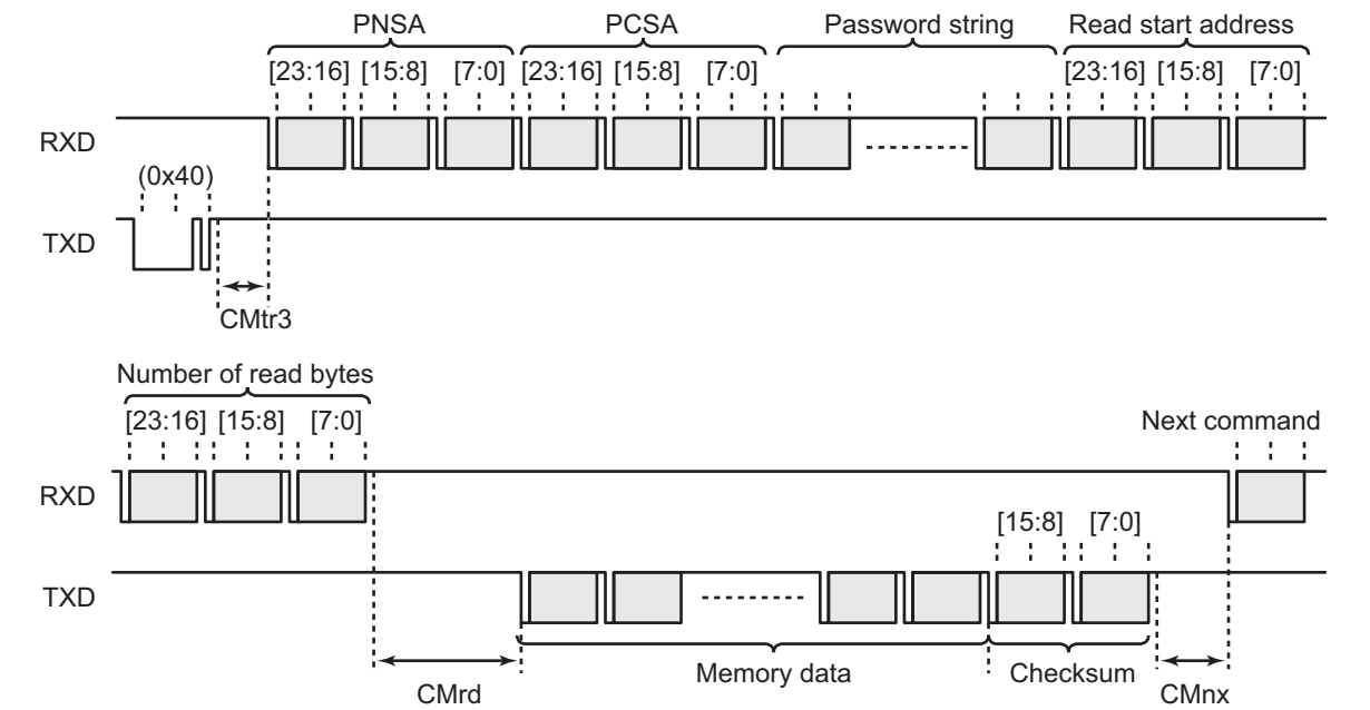
Figure 22-9 Flash Memory Read Command
