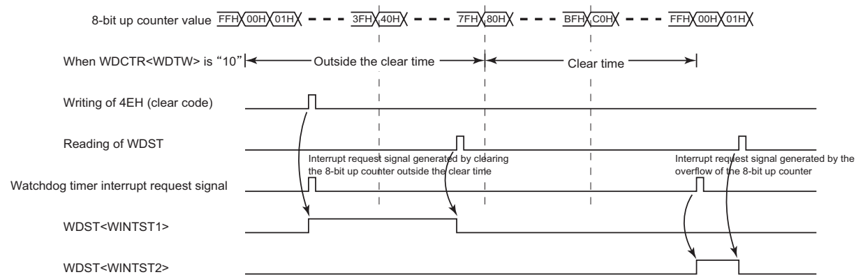
Figure 5-4 Changes in the Watchdog Timer Status
