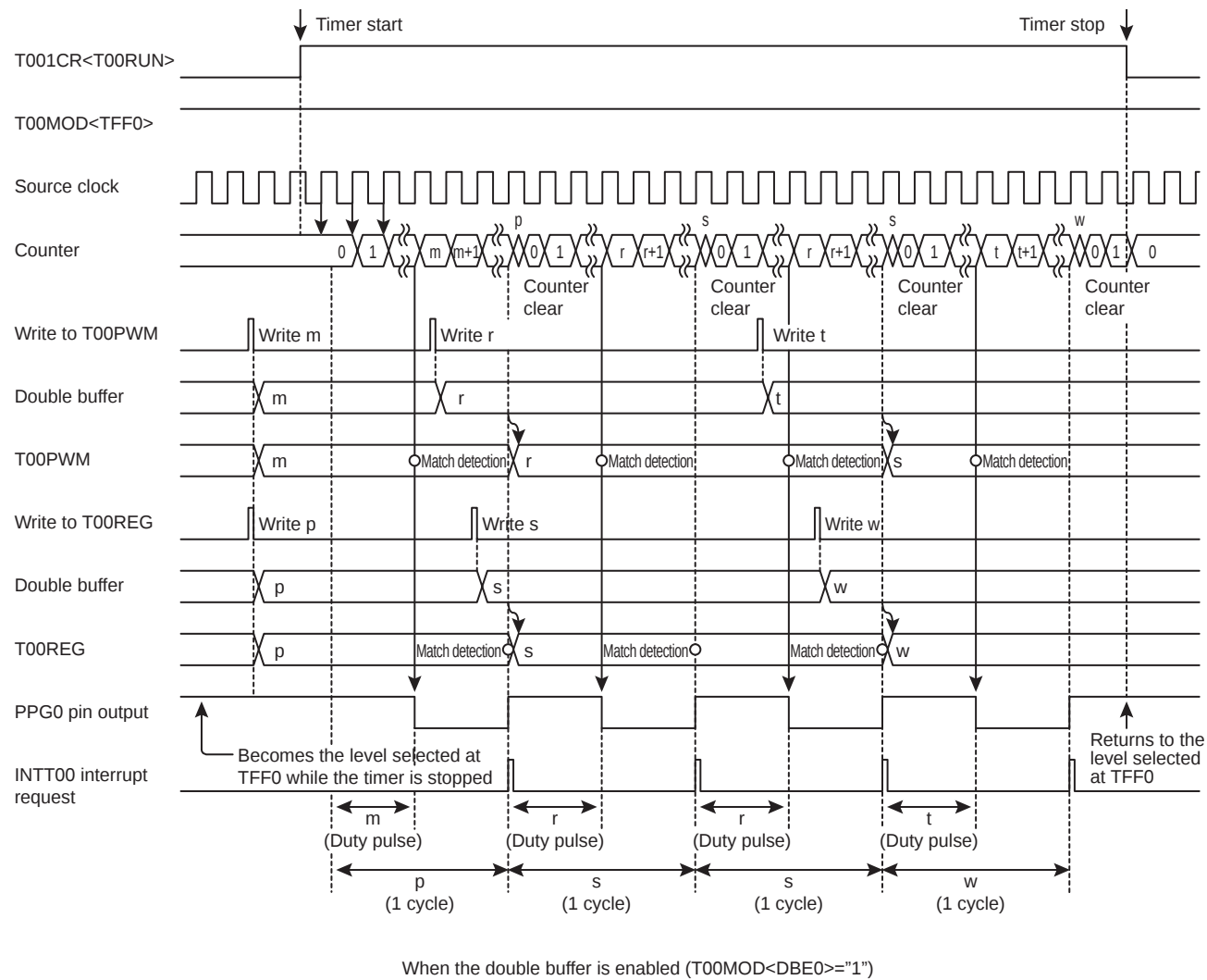
Figure 14-9 8-bit PPG Mode Timing Chart
