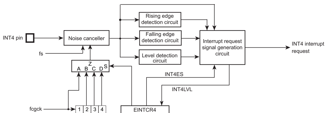
Figure 4-3 External Interrupt 4
