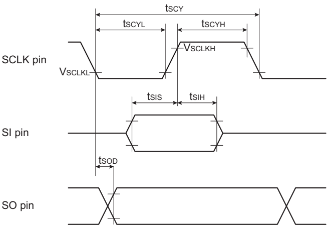
Figure 17-16 AC Characteristics
