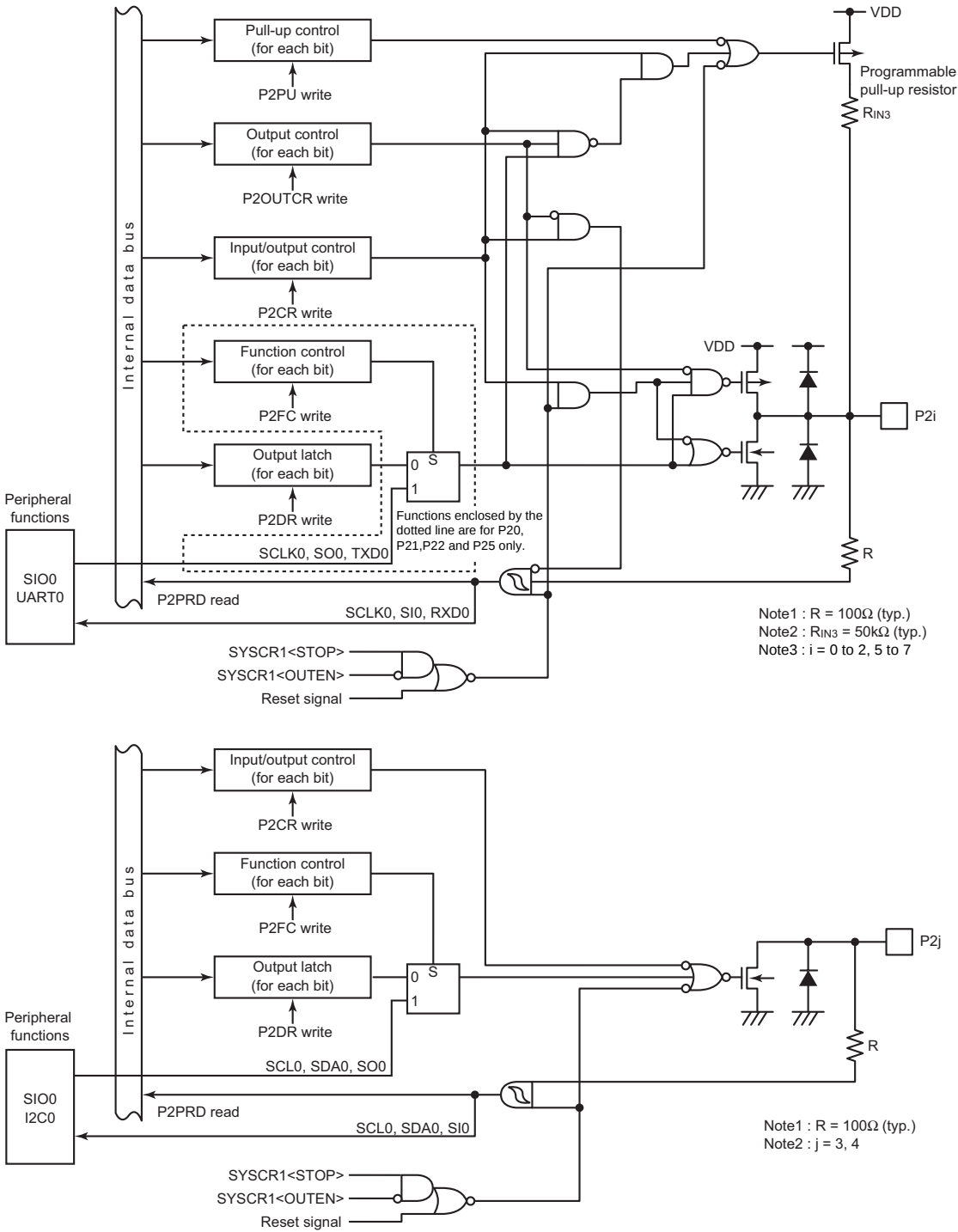
Figure 8-5 Port P2
