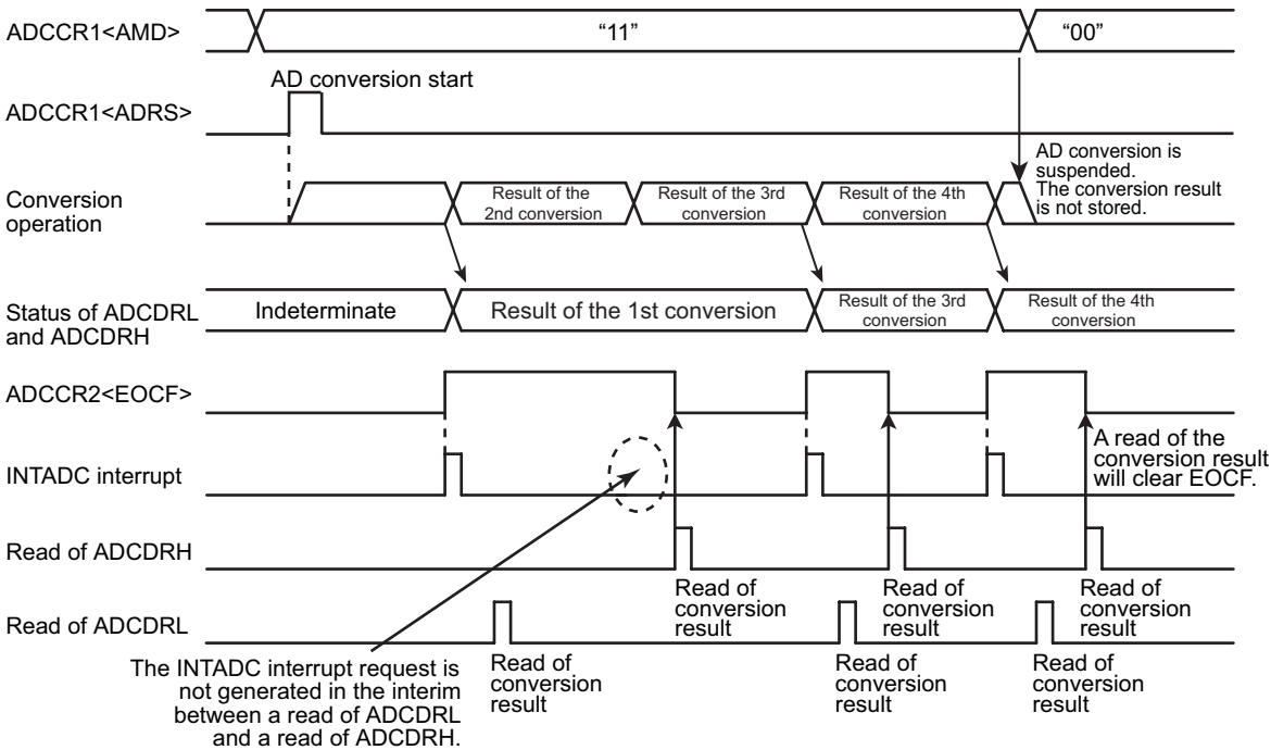
Figure 20-3 Repeat Mode
