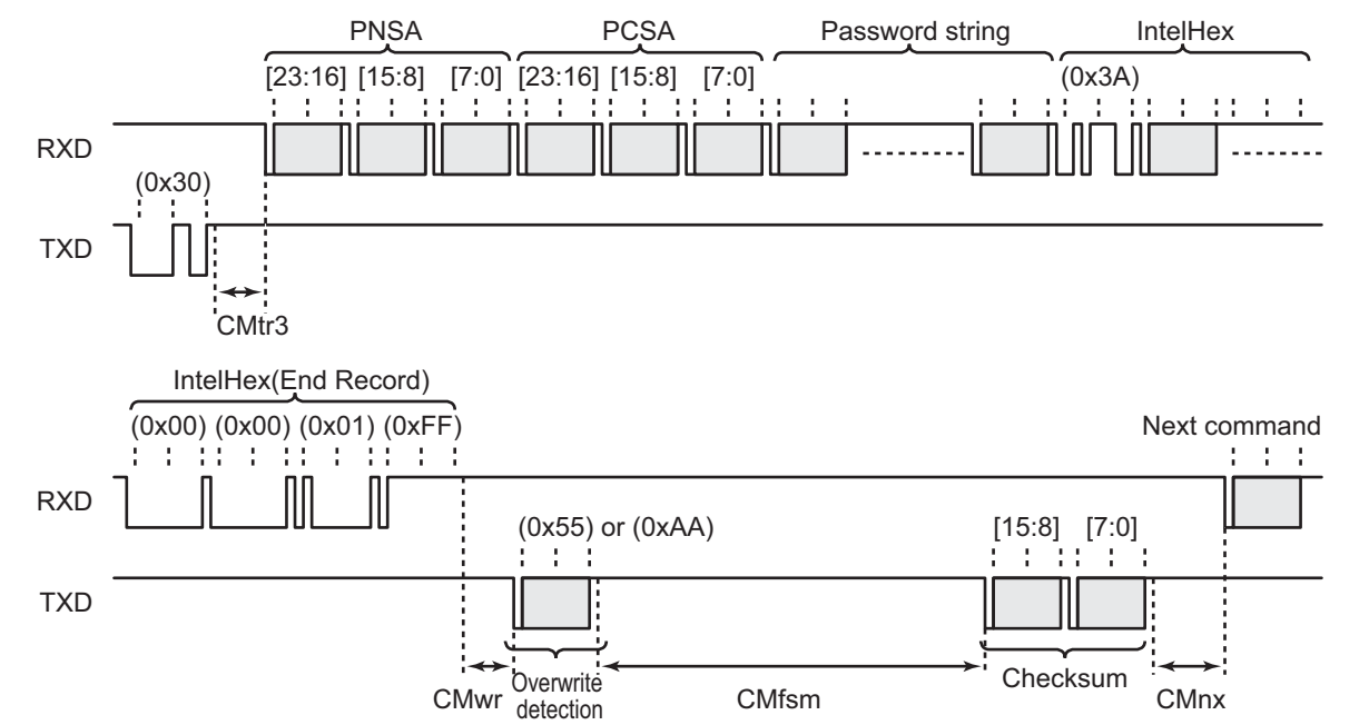
Figure 22-8 Flash Memory Write Command
