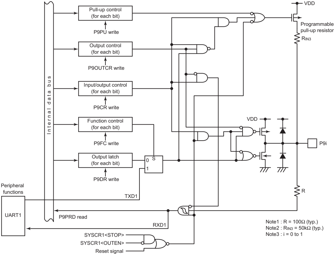
Figure 8-9 Port P9
