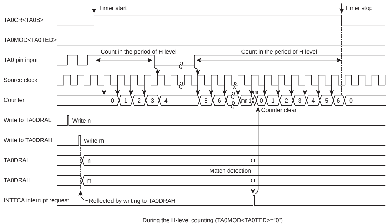
Figure 13-6 Window Mode Timing Chart
