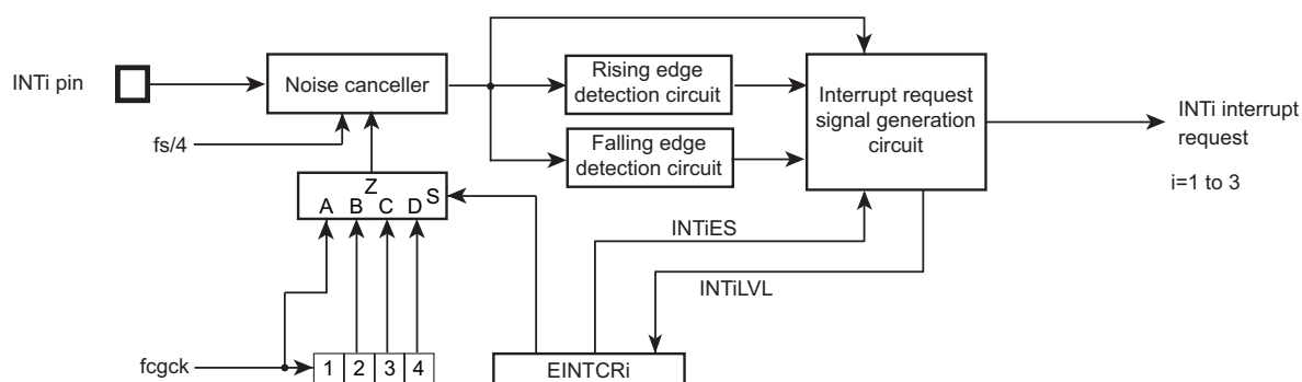
Figure 4-2 External Interrupts 1/2/3
