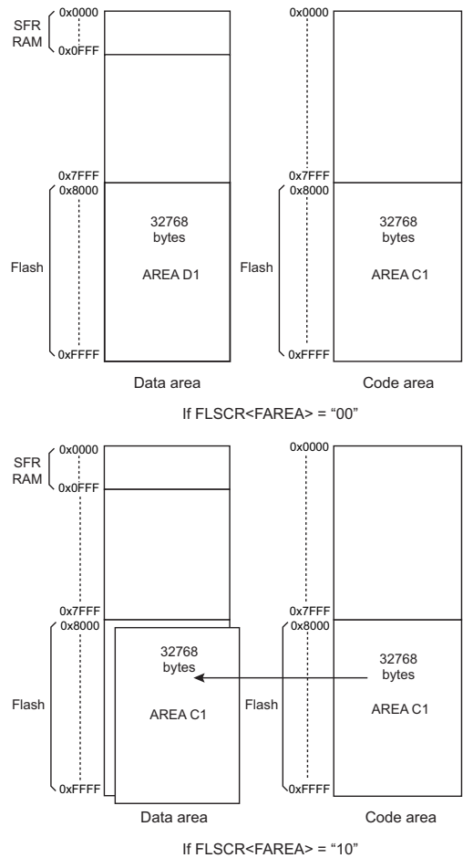
Figure 21-1 Area Switching Using the FLSCR1<FAREA> Setting
