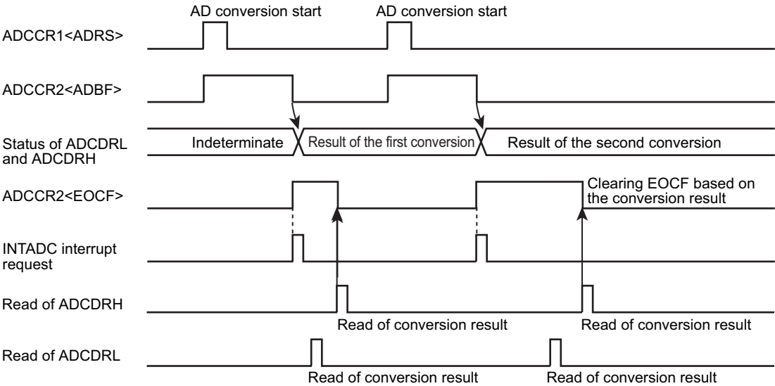
Figure 20-2 Single Mode
