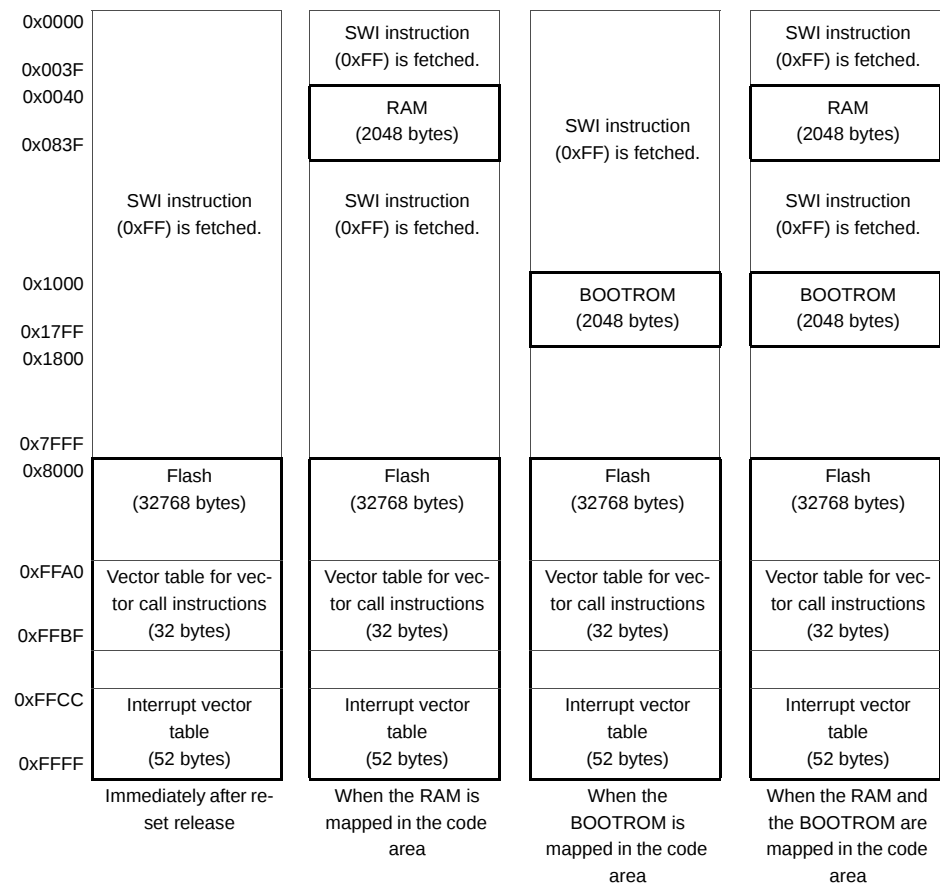
Figure 2-1 Memory Map in the Code Area
