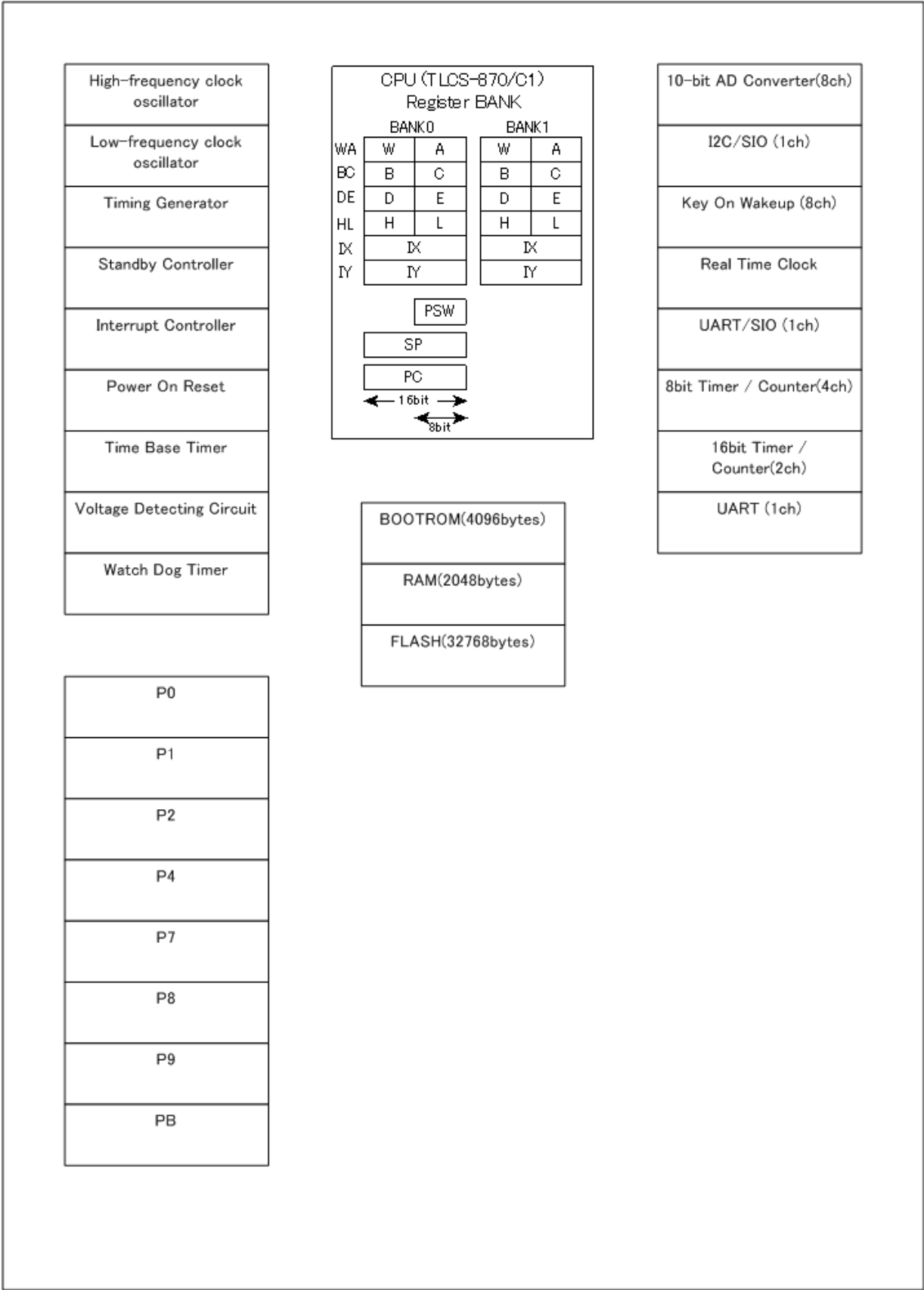
Figure 1-2 Block Diagram
