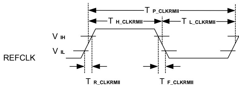
Figure 4: Clock Timing RMIl
