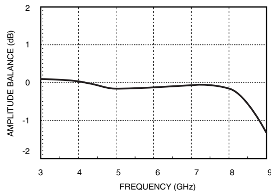
Amplitude Balance
