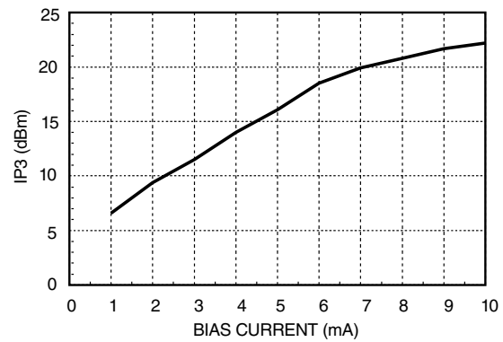
Input Third Order Intercept vs Bias at 6 GHz
