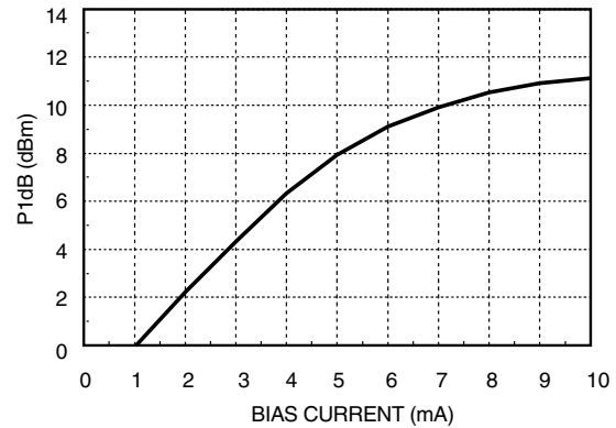
Input Compression vs Bias at 6 GHz
