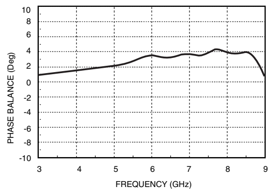
Phase Balance
