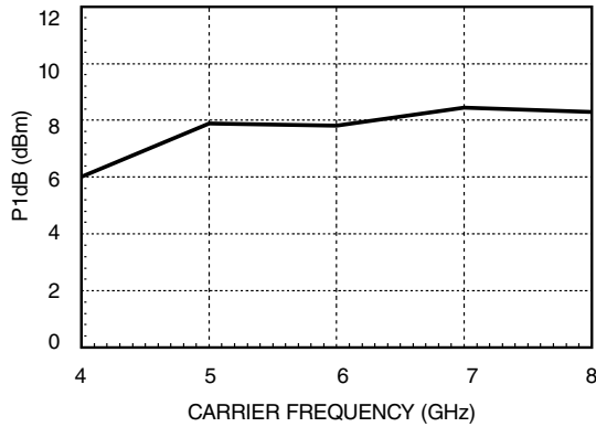
Input Compression vs Frequency *
