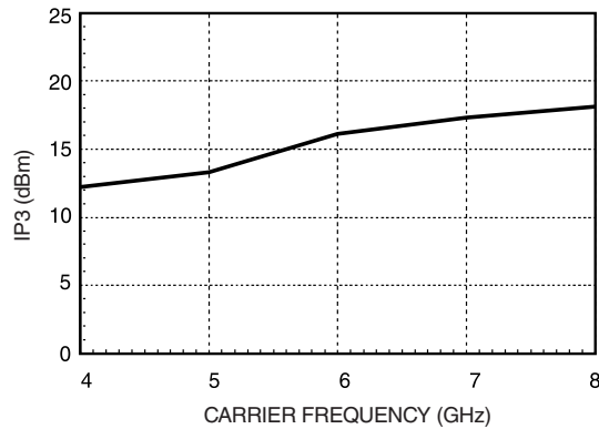
Input Third Order Intercept vs Frequency *
