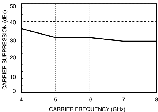
Carrier Suppression *
