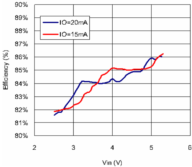
Efficiency vs. Vin (Driving 3WLEDs)
