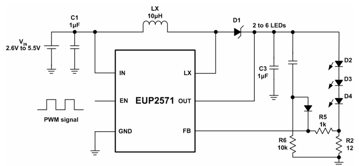
Figure 6. Recommended Soft-Start Circuit
