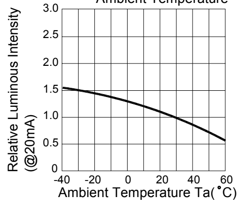
Fig.3 Relative Luminous Intensity VS. Ambient Temperature
