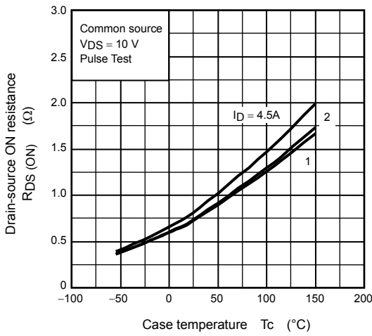
R_{DS(ON)} - T_c
