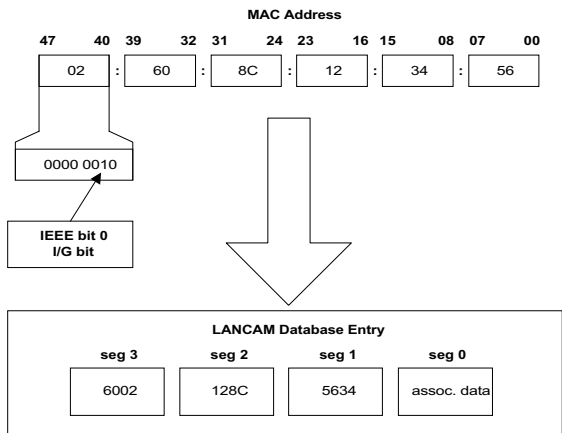
Figure 5: MAC Address Byte Order
