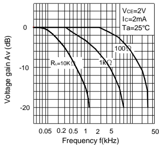
Fig. 10 Frequency Response
