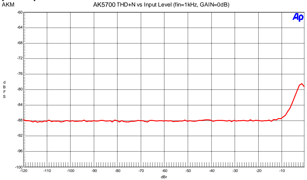
Figure 1. THD+N vs. Input Level
